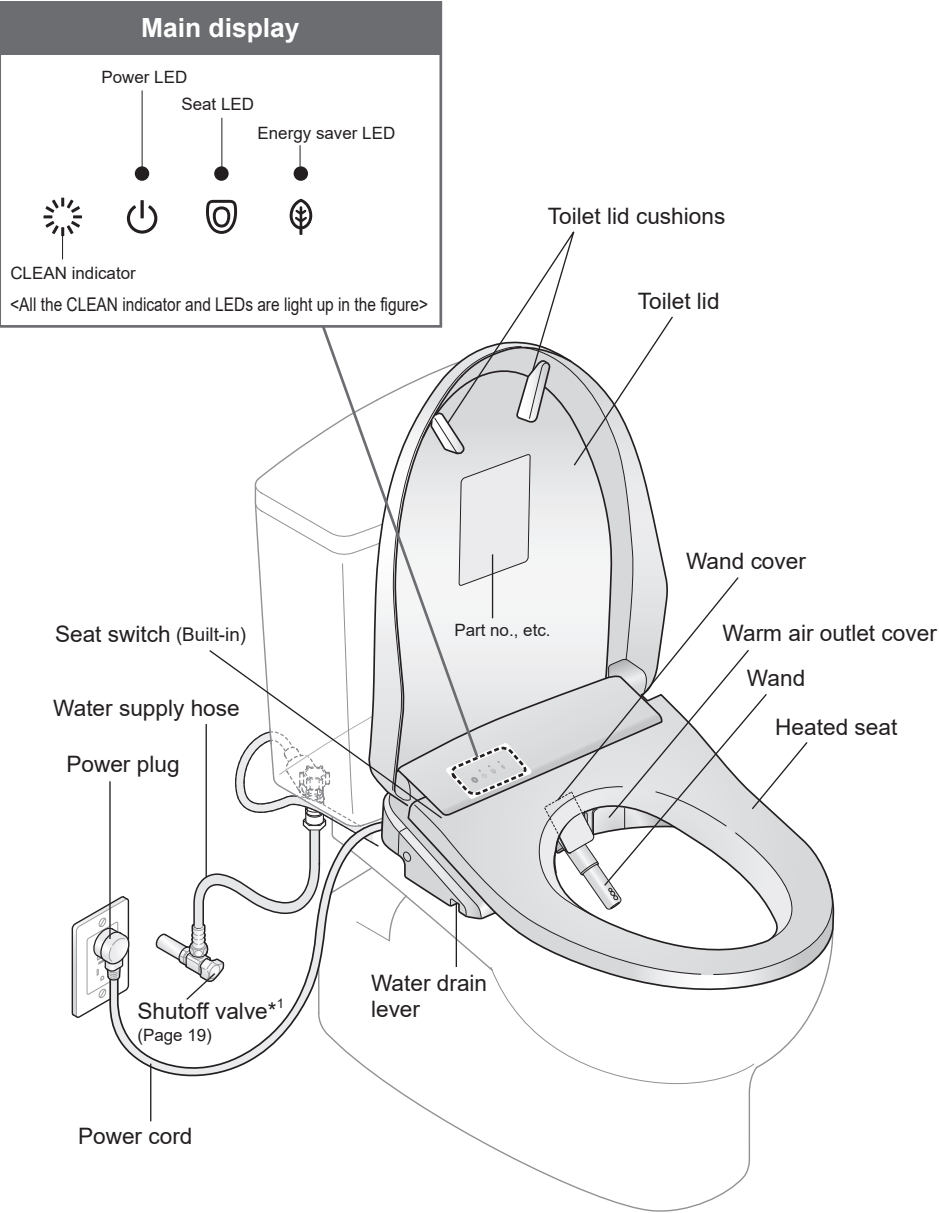
<Illustration shows SW3054>
